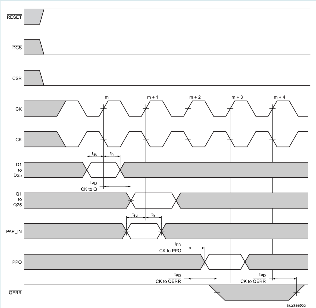
Fig 7. Timing diagram for SSTUM32866 used as a single device; C0 = 0, C1 = 0
